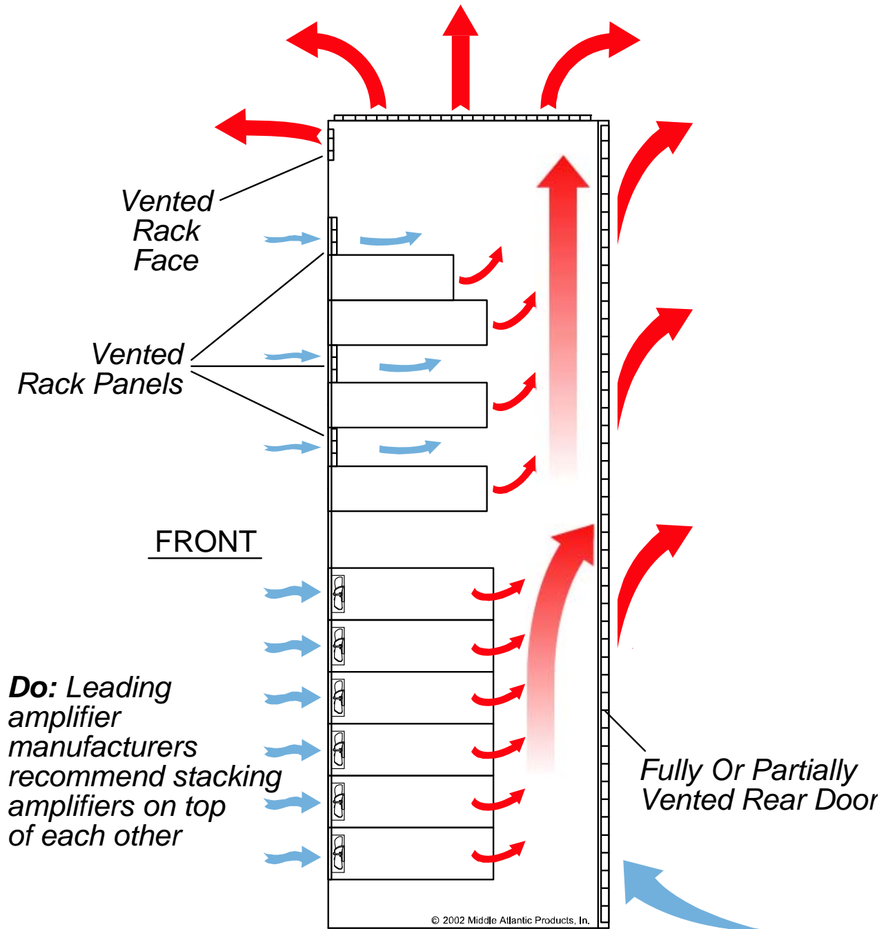
SIDE VIEW
